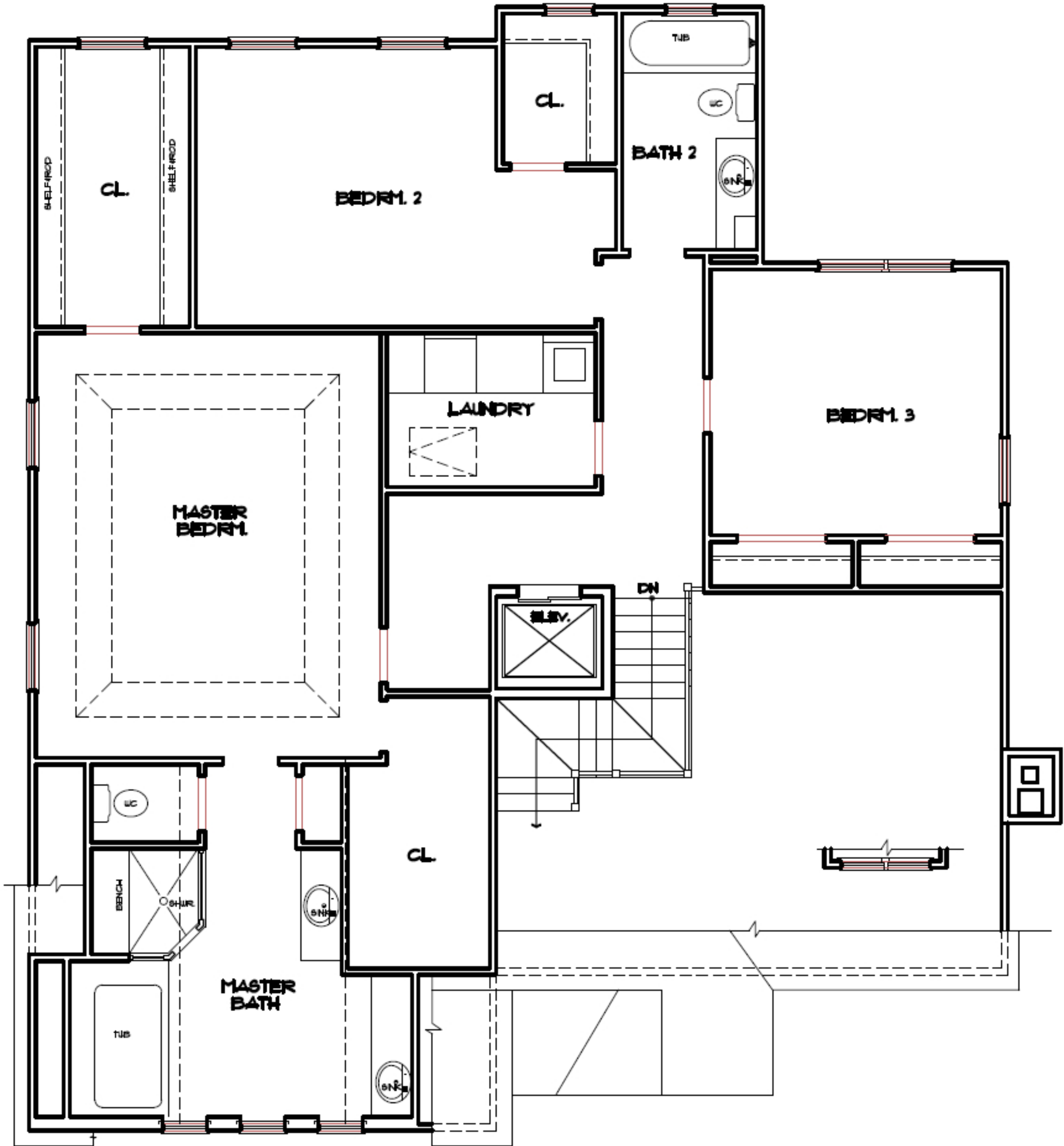
SECOND FLOOR
